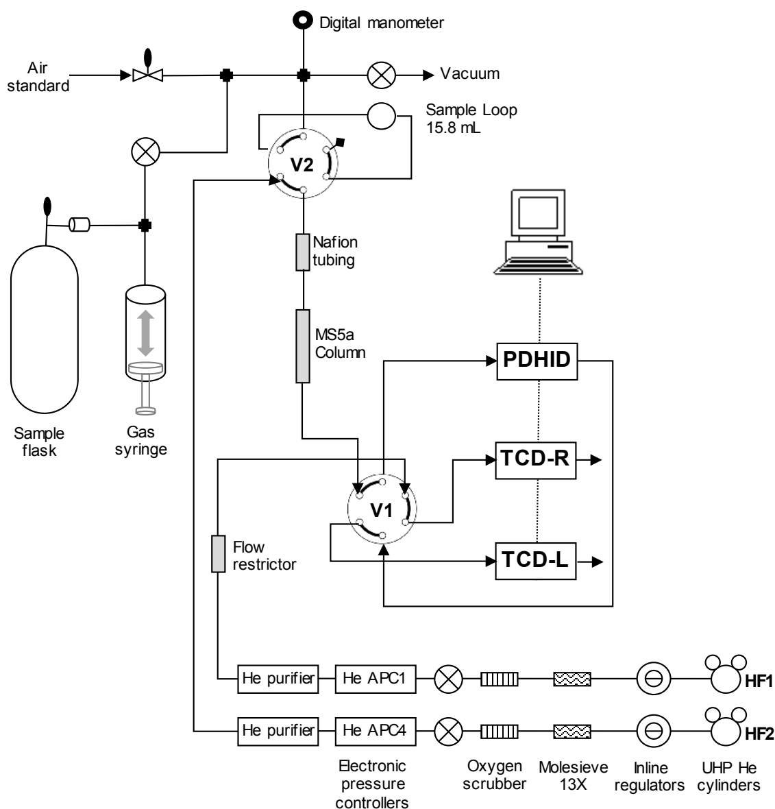
Figure 2.1: Schematic of the analytical set-up of the neon measurement system.
