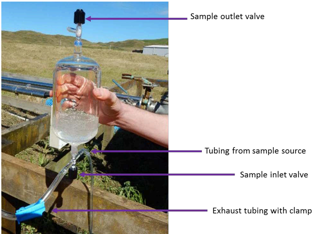
Figure 3.1 Annotated photograph of the neon sample flask.
