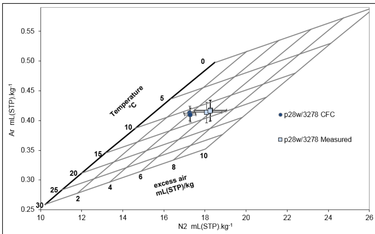
Figure 4.6 Comparison of the measured Ar and N 2 concentrations measured simultaneously with the Ne measurement (square symbols) at well P28w/3278 to the Ar and N 2 concentrations measured during CFC analysis (circle symbols). The error bars represent measurement uncertainty calculated according to Equation 4.
