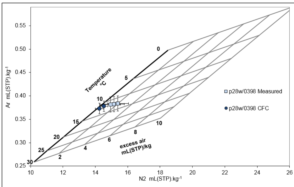
Figure 4.7 Comparison of the measured Ar and N 2 concentrations measured simultaneously with the Ne measurement (square symbols) at well P28w/0398 to the Ar and N 2 concentrations measured during CFC analysis (circle symbols). The error bars represent measurement uncertainty calculated according to Equation 4.
