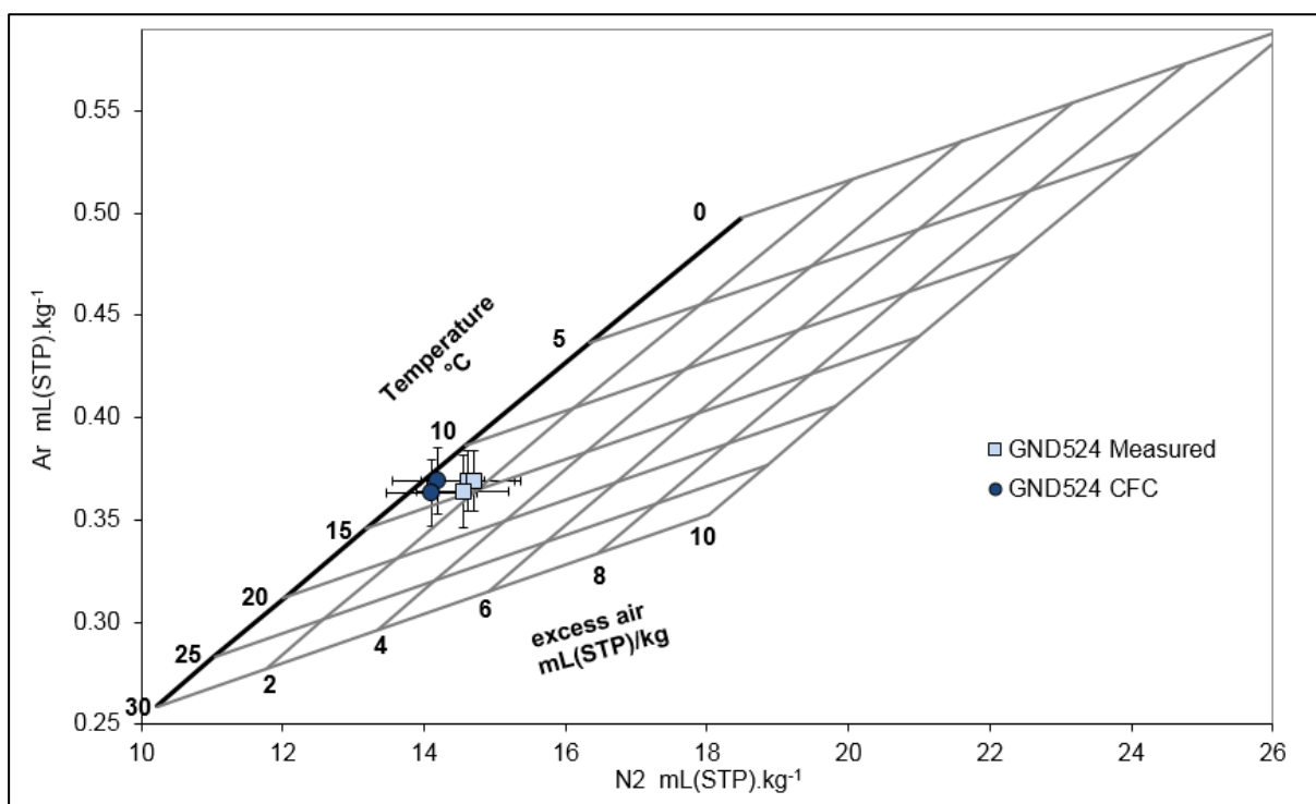
Figure 4.5 Comparison of the measured Ar and N 2 concentrations measured simultaneously with the Ne measurement (square symbols) at well GND524 to the Ar and N 2 concentrations measured during CFC analysis (circle symbols). The error bars represent measurement uncertainty calculated according to Equation 4.
