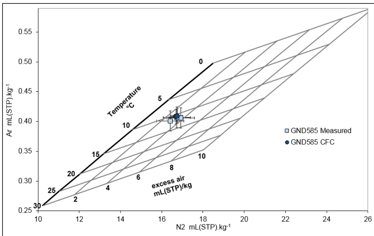
Figure 4.4 Comparison of the measured Ar and N 2 concentrations measured simultaneously with the Ne measurement (square symbols) at well GND585 to the Ar and N 2 concentrations measured during CFC analysis (circle symbols). The error bars represent measurement uncertainty calculated according to Equation 4.
