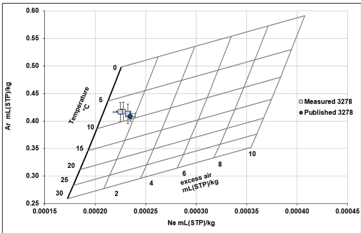
Figure 4.3 Comparison of the measured Ne and Ar concentrations (square symbols) at well P28w/3278 to Seltzer et al. (2015) published result (circle symbols). The error bars represent measurement uncertainty calculated according to Equation 4.
