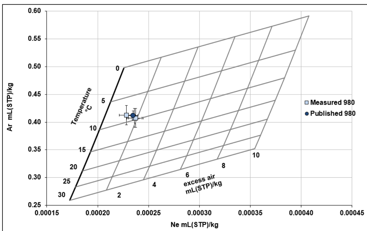
Figure 4.2 Comparison of the measured Ne and Ar concentrations (square symbols) at well P28w/0980 to Seltzer et al. (2015) published result (circle symbols). The error bars represent measurement uncertainty calculated according to Equation 4.
