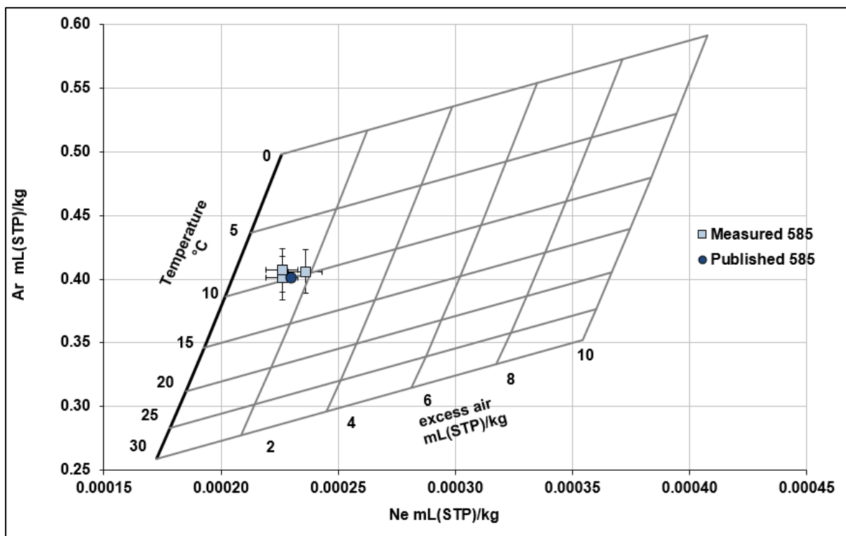
Figure 4.1 Comparison of the measured Ne and Ar concentrations (square symbols) at well GND585 to Seltzer et al. (2015) published result (circle symbols). The error bars represent measurement uncertainty calculated according to Equation 4.
