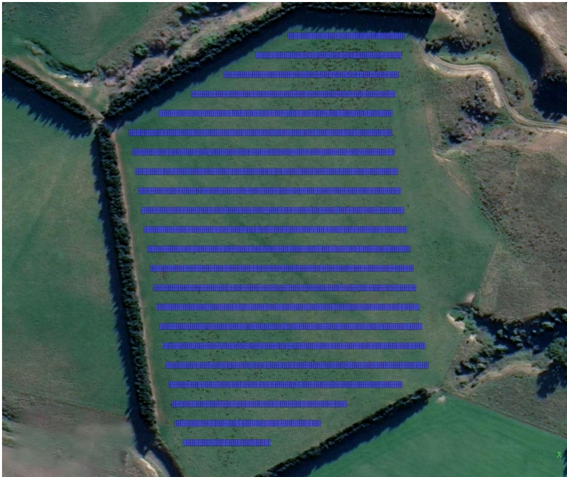
Figure 12. View of the fixed-tilt arrangement 1 .
