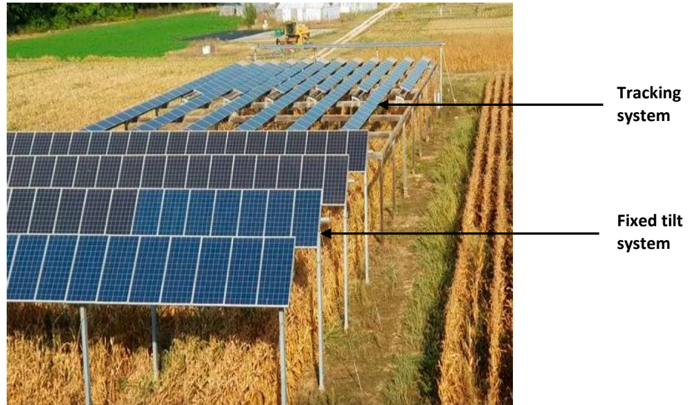
Figure 4. Fixed tilt and tracking systems (Toledo & Scognamiglio, 2021).
